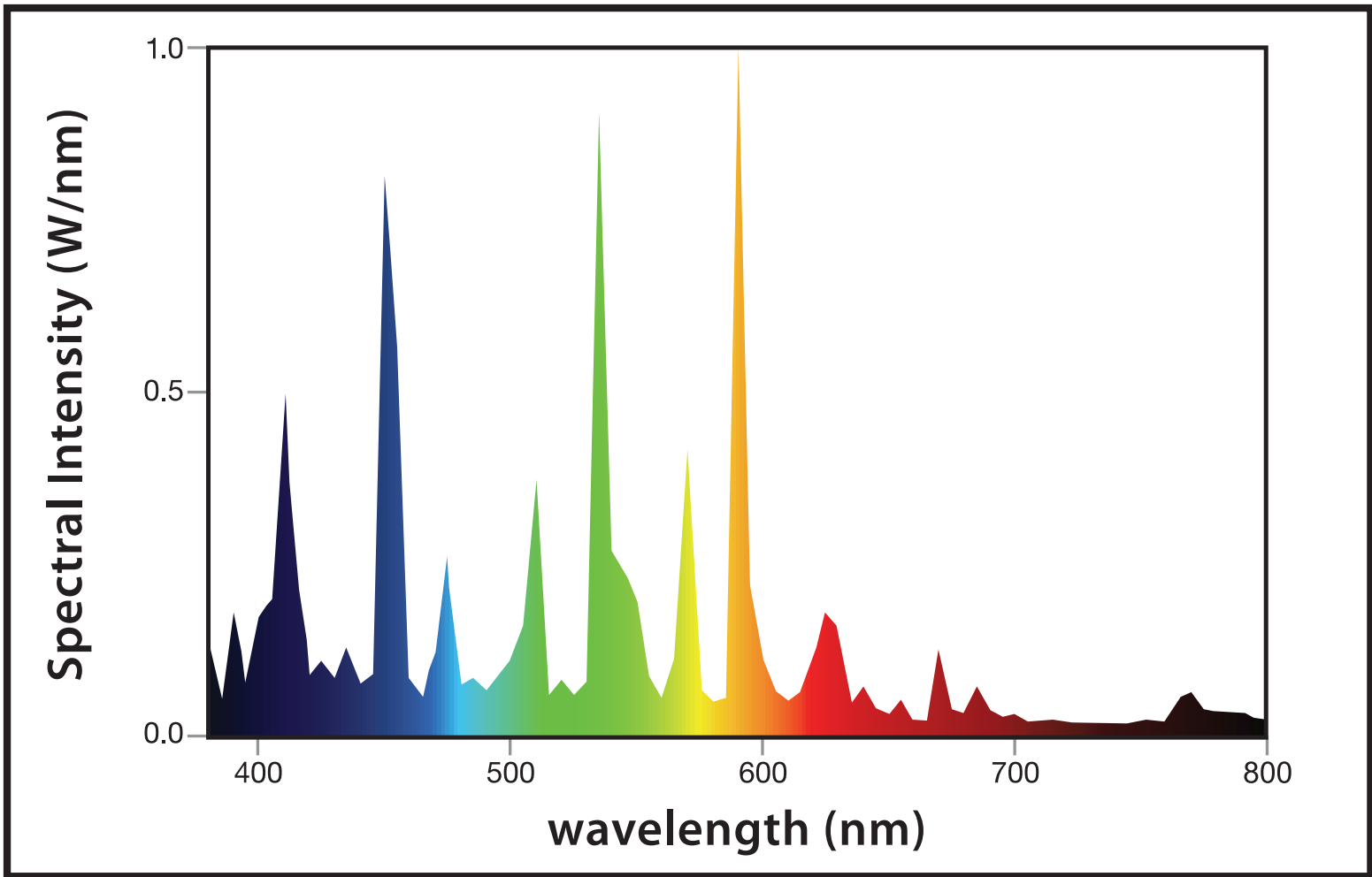
Ultra Sun 600 Watt - MH Conversion Lamp - Spectral Intensity Graph
